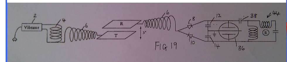
CORREA PAGD SYSTEM ( P ulsed A bnormal G low D ischarge) =>
